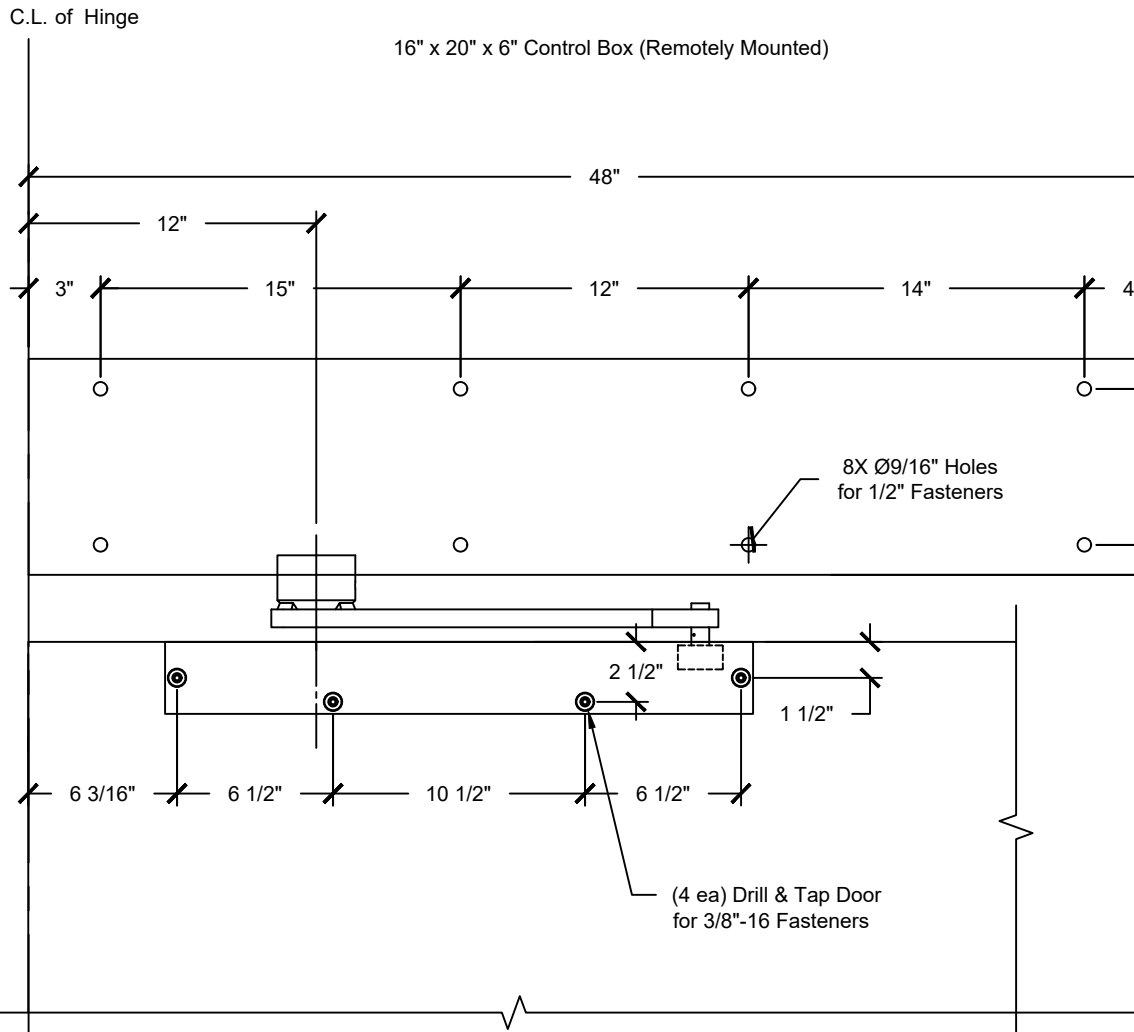
1 Elevation: 1502-3 Right Hand Pull to Open
