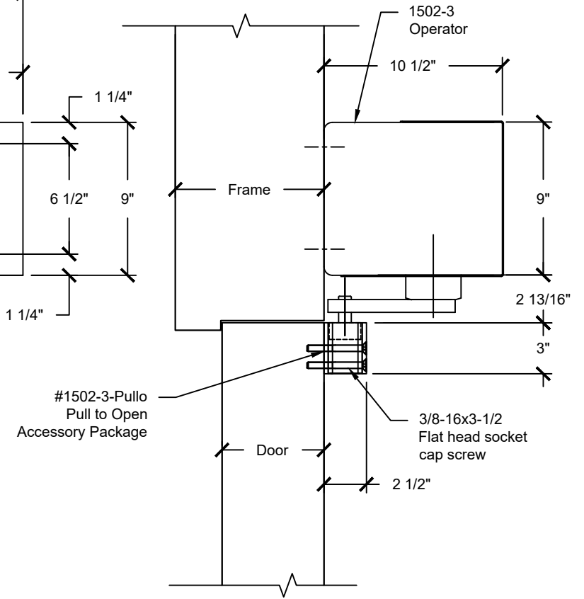
2 Section Head Detail: 1502-3
